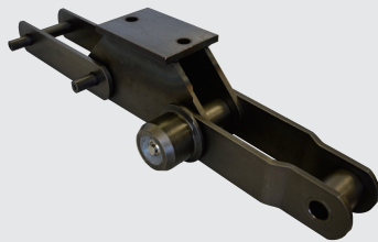
RECLAIMER CHAIN
